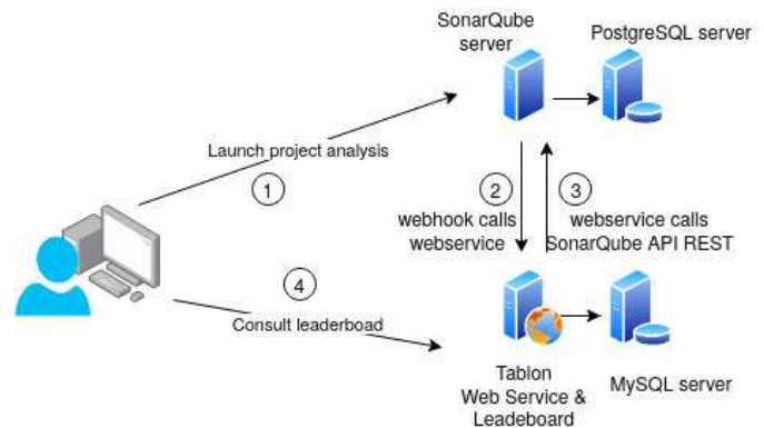
Fig. 2. Contest implementation environment
