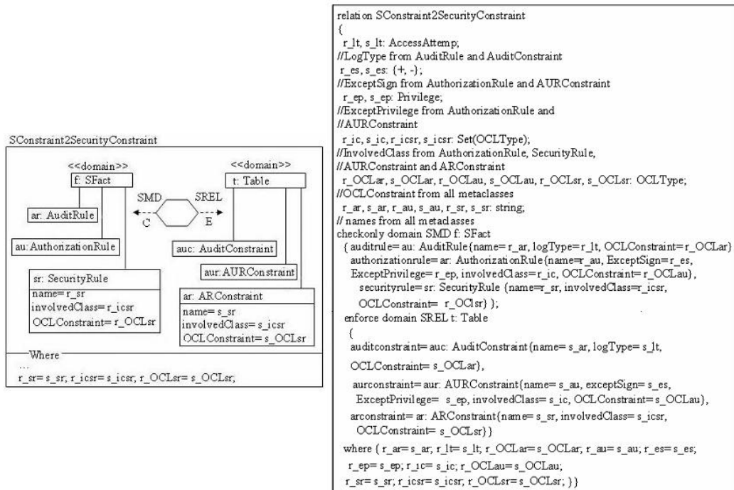
Figura 7. Transformando SConstraint en SecurityConstraint
