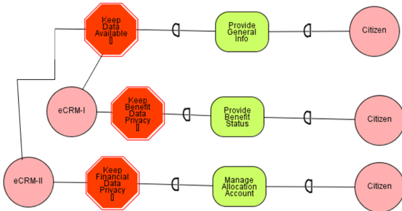
Fig. 4. Part of the SEAD of the instantiated applications of the eCRM (SPL) – (Late Requirements phase).
