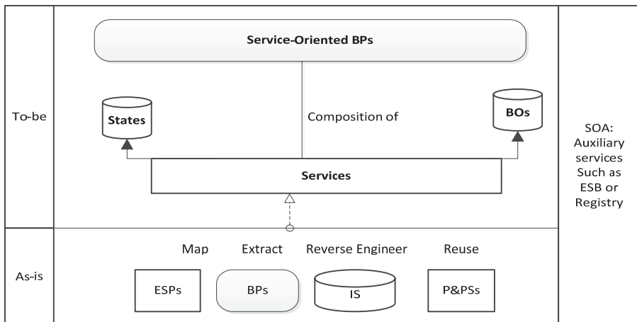
Fig. 1. Techniques to transform as-is BP into service-oriented BP.
