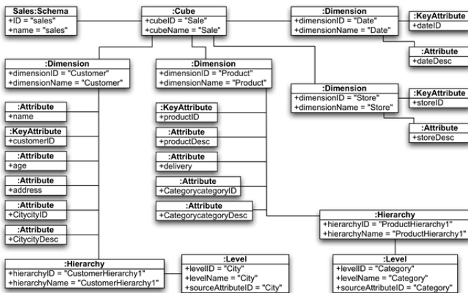
Fig. 6. Logical Model (PSM). Dimensions’ structure.
