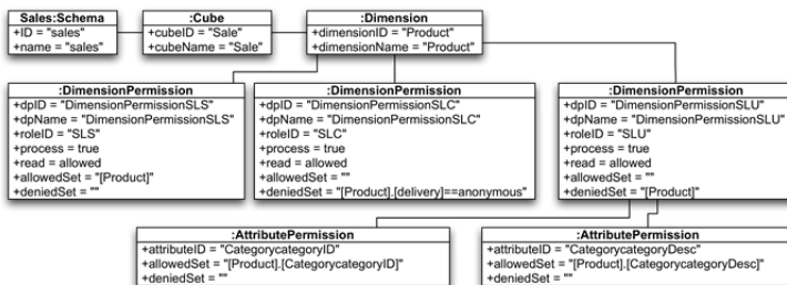
Fig. 7. Logical Model (PSM). Product dimension’s security rules.
