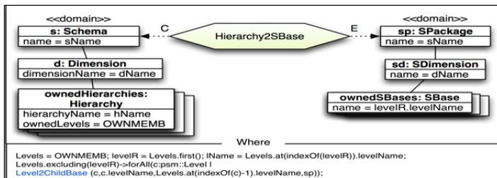
Fig. 4. Hierarchy2SBase relation.
