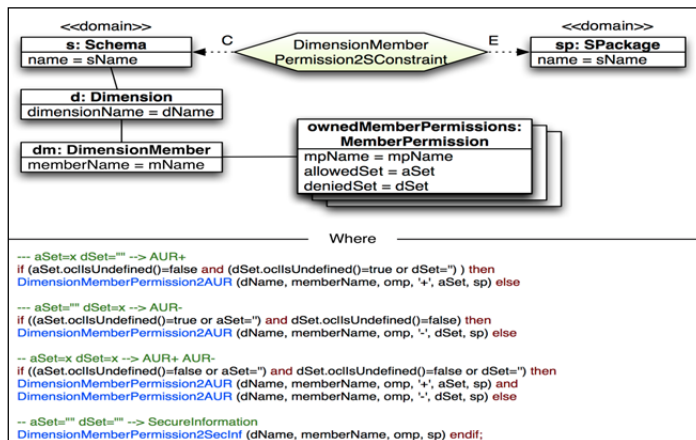
Fig. 5. DimensionMemberPermission2SConstraint relation.
