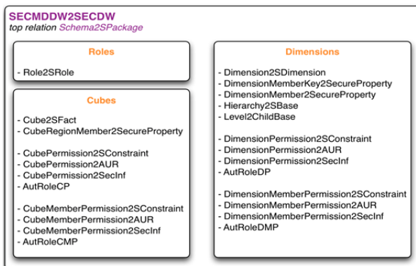
Fig. 3. A reverse engineering process for legacy OLAP applications.
